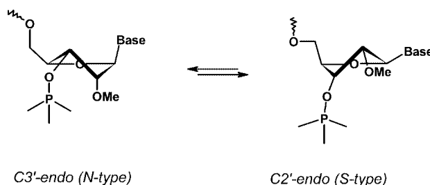
Figure 1. Representations of the S -type (DNA-like) and N -type (RNA-like) structures of the sugar conformations.
