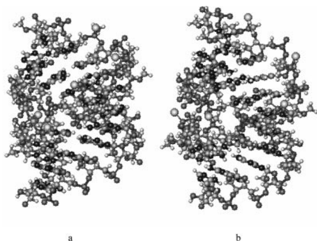
Figure 3. Energy-minimized structures of the hybrid duplexes a) ( R_P,R_P,R_P,R_P,R_P )- 2e /RNA and b) ( S_P,S_P,S_P,S_P,S_P )- 2f /RNA. The duplex structures were generated with the HyperChem 7.5 molecular modelling program [49] and optimized using the AMBER96 force field method with default parameters. [50]
