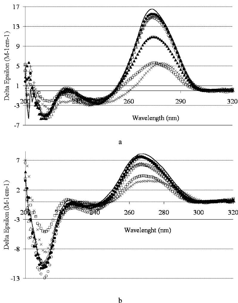
Figure 2. Circular dichroism (CD) spectra of a) free single strands of oligonucleotides 2 : 2a (●), 2b (+), 2c (○), 2d (Δ), 2e (▲), 2f (□), 11 (×), and 12 (–); b) heteroduplexes of chimeric oligonucleotides 2 with RNA 10 : 2a /RNA (●), 2b /RNA (+), 2c /RNA (○), 2d /RNA (Δ), 2e /RNA (▲), 2f /RNA (□), 11 /RNA (×), and 12 /RNA (–). Reagents and conditions: 10 mM Tris-HCl, 100 mM NaCl, and 10 mM MgCl 2 (pH = 7.4), T = 20 °C, concentration = 4 μM. See Table 1 for base sequences of the corresponding oligonucleotides.
